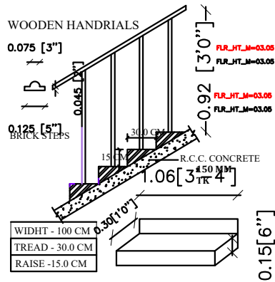
STAIRCASE DETAILS
