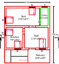
PROPOSED FIRST FLOOR PLAN
