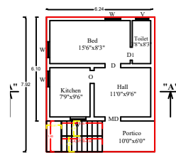
EXISTING GROUND FLOOR PLAN
