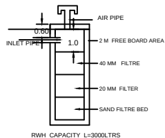
RWH_CAPACITY_L=3000LTRS
