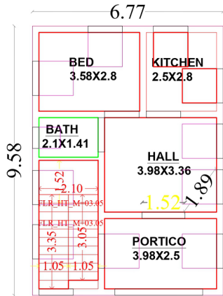
GROUND FLOOR PLAN (FACEING OF EAST)
