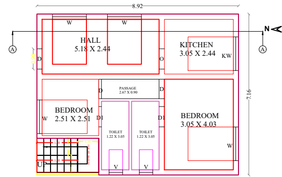
GROUND FLOOR PLAN (NORTH FACING)
