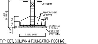
TYP. DET. COLUMN & FOUNDATION FOOTING
