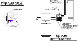
STAIRCASE DETAIL
