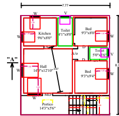
PROPOSED GROUND FLOOR PLAN
