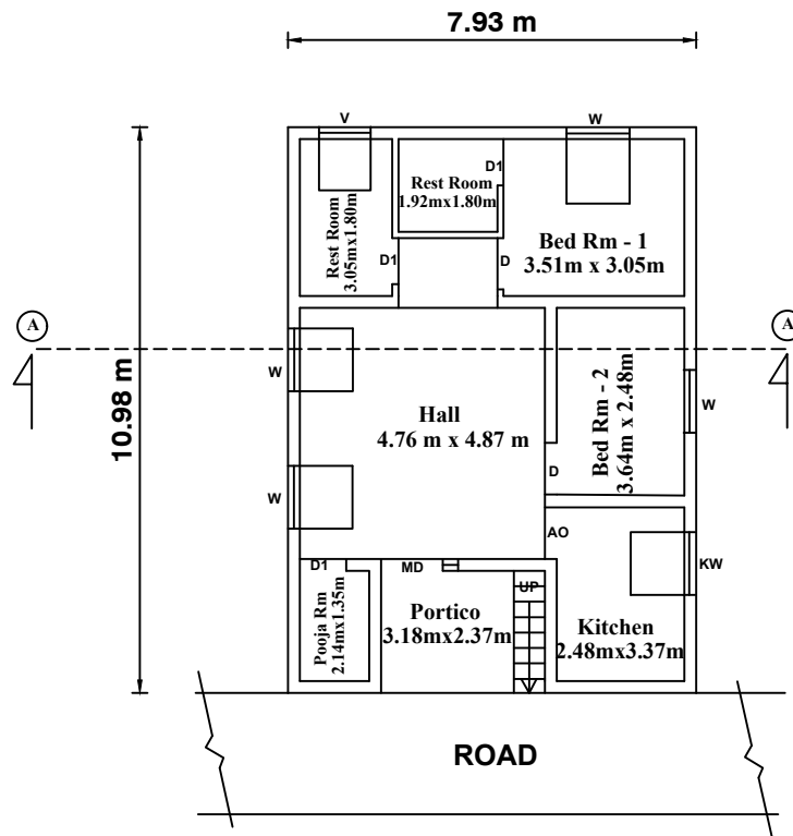
EXISTING GROUND FLOOR PLAN SOUTH FACING
