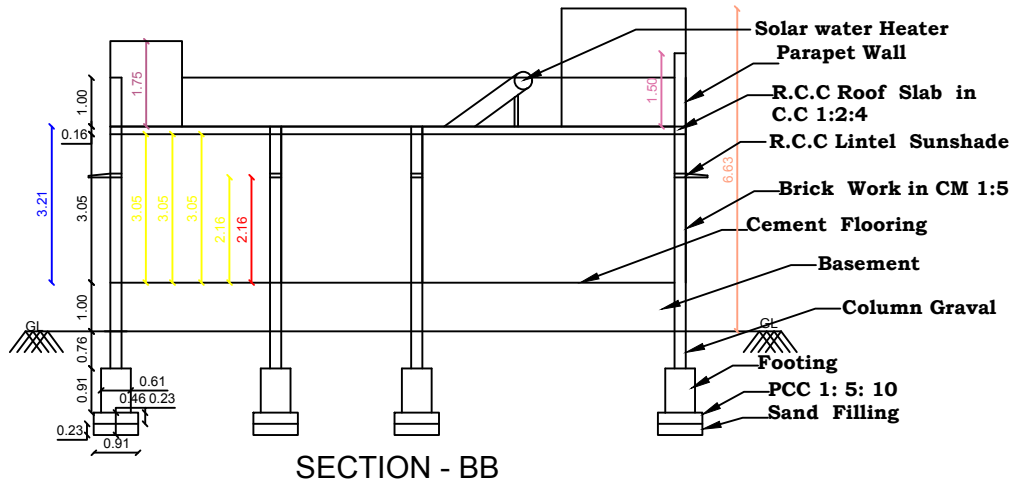
SECTION - BB
