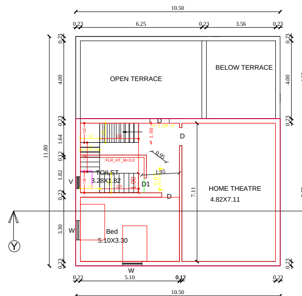
SECOND FLOOR PLAN PROPOSED BUILDING
