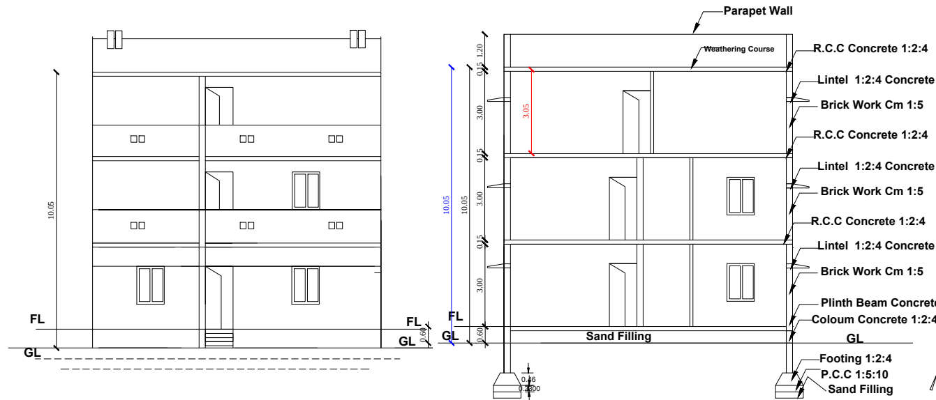
FRONT ELEVATION
