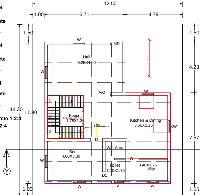
GROUND FLOOR PLAN EXISTING BUILDING
