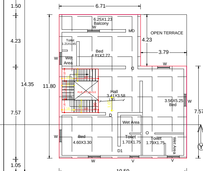
FIRST FLOOR PLAN EXISTING BUILDING
