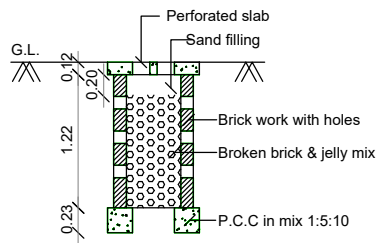
PERCOLATION PIT
