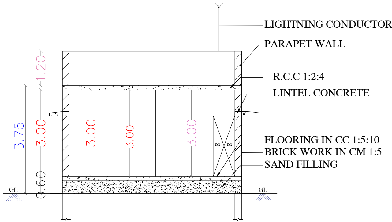
SECTION AB
