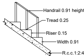
STAIECASE DETAILS
