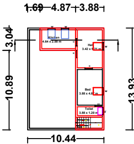
Existing First Floor Plan
