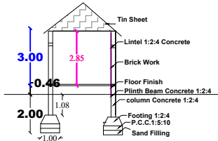
SECTION SECTION ON - AA
