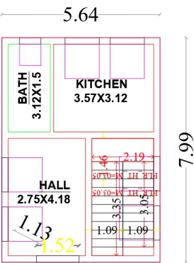
FIRST FLOOR PLAN (FACEING OF NORTH)
