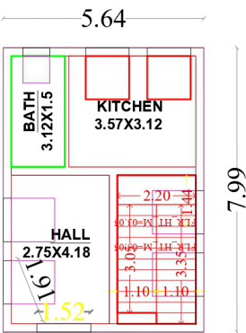
GROUND FLOOR PLAN (FACEING OF NORTH)
