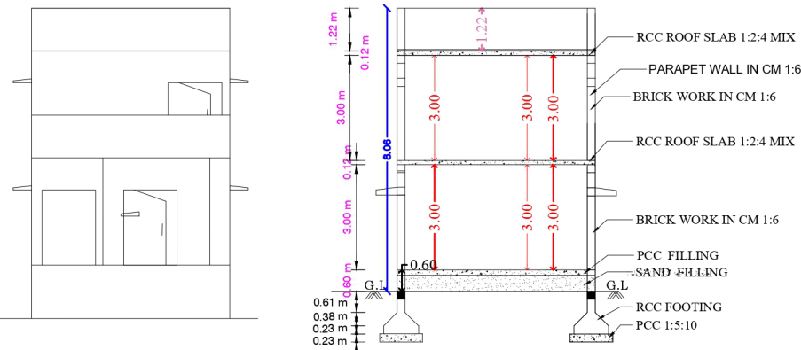
FRONT ELEVATION (FACEING OF NORTH)
