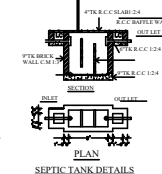
SEPTIC TANK DETAILS SCALE 1"=8'
