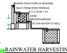
RAINWATER HARVESTING
