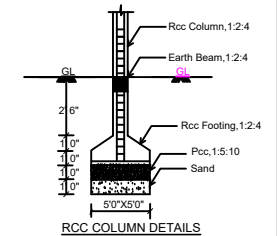
RCC COLUMN DETAILS
