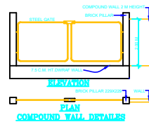
PLAN COMPOUND WALL DETAILS
