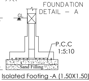
Isolated Footing - A (1.50X1.50)
