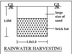
RAINWATER HARVESTING
