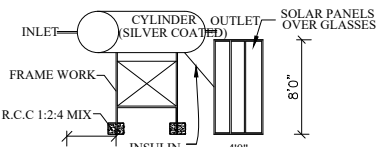
Waste Water Recycle Unit Not To Scale
