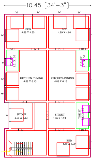
SECOND FLOOR PLAN (WEST FACING)
