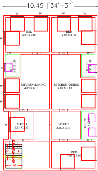
FIRST FLOOR PLAN (WEST FACING)
