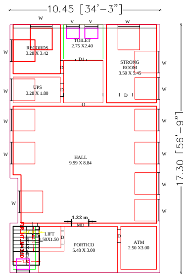
GROUND FLOOR PLAN (WEST FACING)
