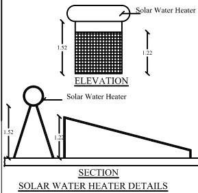
SOLAR WATER HEATER DETAILS
