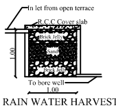
RAIN WATER HARVEST
