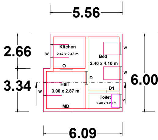
Ground Floor Plan (North Facing)
