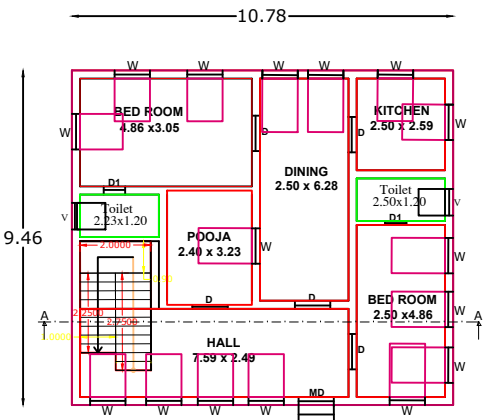
GROUND FLOOR PLAN ( SOUTH FACING)
