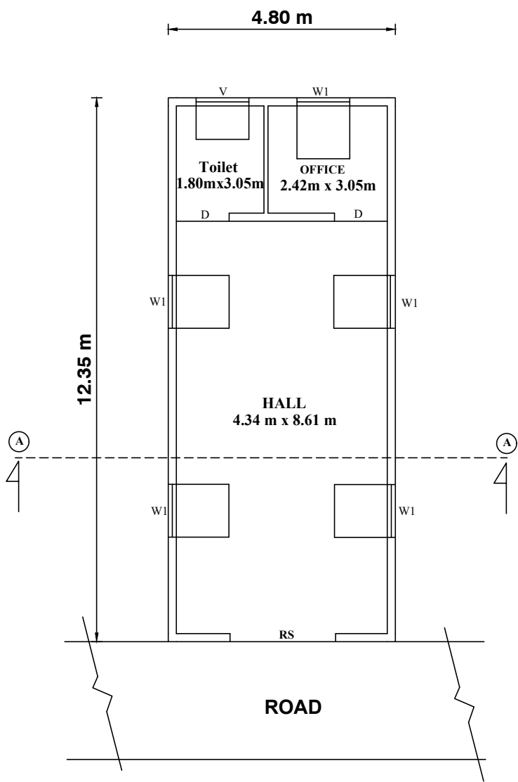
PROPOSED GROUND FLOOR PLAN WEST FACING
