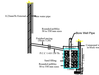
RWH CAPACITY L=2000 LITTER
