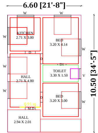
GROUND FLOOR PLAN NORTH FACING
