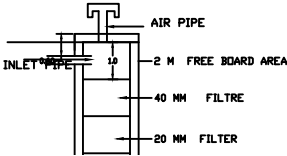
20 MM FILTER
