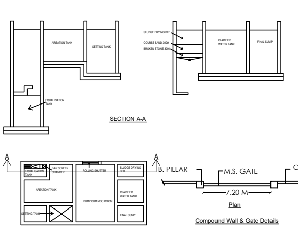
SEWAGE TREATMENT PLANT PLAN
