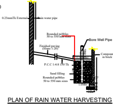
PLAN OF RAIN WATER HARVESTING
