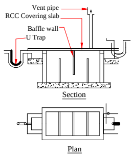
Section
