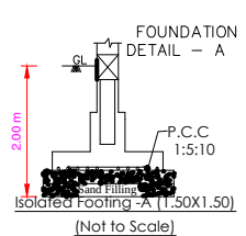
FOUNDATION DETAIL - A
