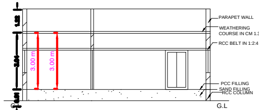
SECTION ON-'AB'
