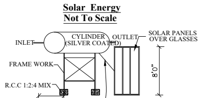
Waste Water Recycle Unit Not To Scale
