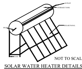
SOLAR WATER HEATER DETAILS NOT TO SCALE
