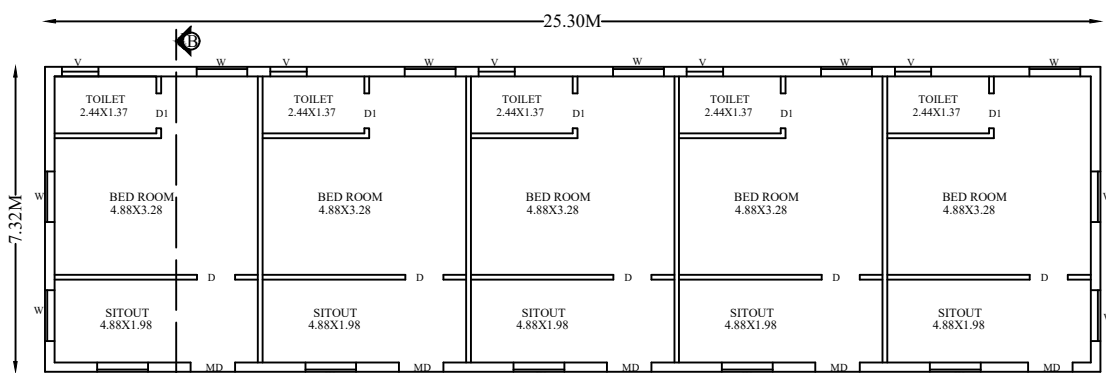
Ext.GROUND FLOOR PLAN
