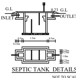
SEPTIC TANK DETAILS NOT TO SCALE
