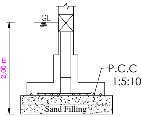
Isolated Footing -A (1.50X1.50) (Not to Scale)
