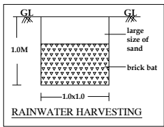
RAINWATER HARVESTING
