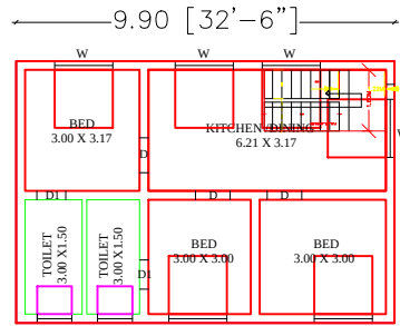
SECOND FLOOR PLAN (WEST FACING)
