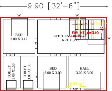
GROUND FLOOR PLAN (WEST FACING)
