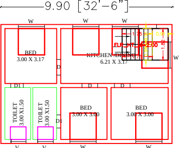
FIRST FLOOR PLAN (WEST FACING)
