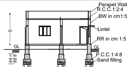
SECTION ON "XX" 8.08
