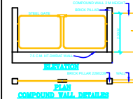
COMPOUND WALL DETAILS
