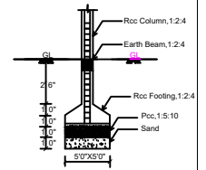
RCC COLUMN DETAILS
