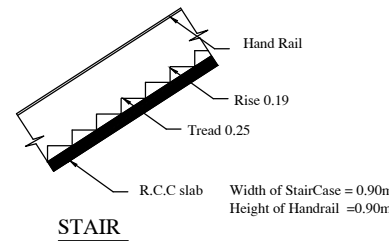
STAIR
