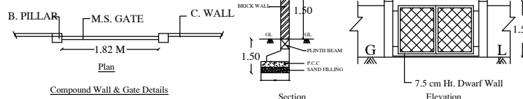
Compound Wall & Gate Details
