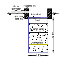
RAIN WATER PERCOLATION PIT
