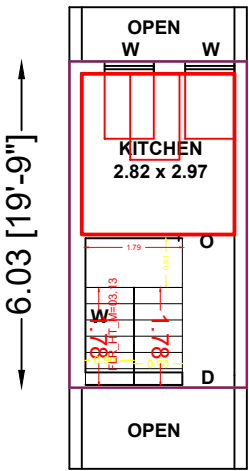
GROUND FLOOR PLAN (EAST FACING)
