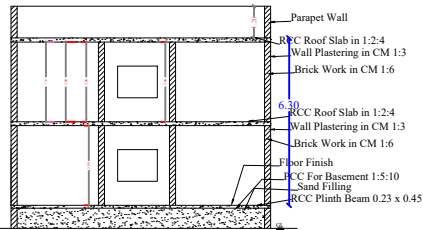
SECTION (N) S.A.
