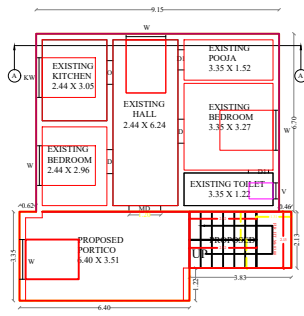
EXISTING AND PROPOSED GROUND FLOOR PLAN (NORTH FACING)
