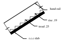
STAIR Width of StairCase = 0.9m
