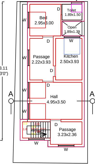
PLAN - F.F-Proposed
