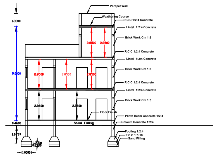
Section
