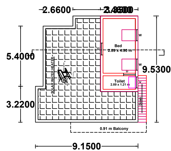
SECOND FLOOR PLAN ( PROPOSED ) & TERRACE FLOOR PLAN
