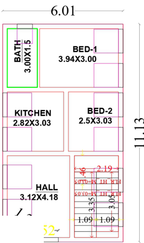
1ST FLOOR PLAN FACEING OF NORTH)
