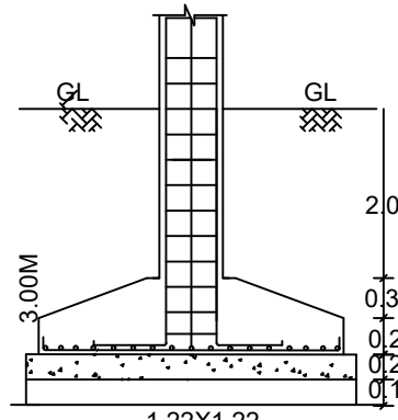
COLUMN DETAILS (NOT TO SCALE) (depends of soil condition)
