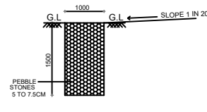
SECTION OF PEBBLE TRENCH SCALE : 1: = 100
