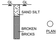
SECTION PERCULATION PIT ( NOT TO SCALE)
