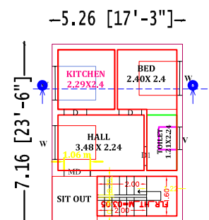
GROUND FLOOR PLAN (NORTH FACING)
