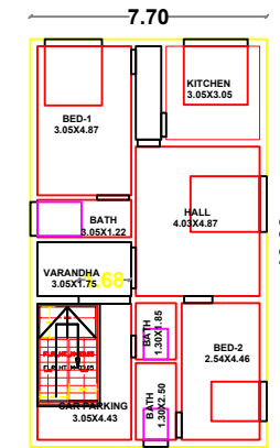
GROUND FLOOR PLAN FACEING OF WEST
