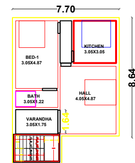
FIRST FLOOR PLAN FACEING OF WEST
