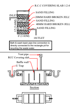
SECTION - 'CD'
