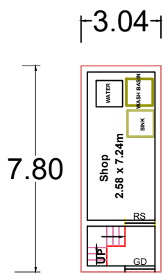
GROUND FLOOR PLAN (EXISTING - COMMERCIAL)
