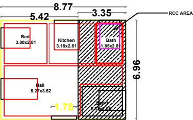
GROUND FLOOR PLAN FACING OF EAST
