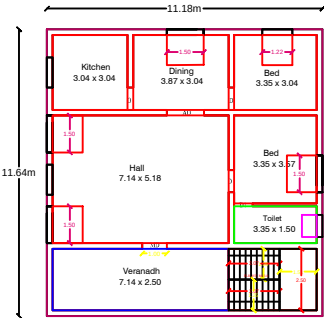
GROUND FLOOR PLAN NORTH FACING
