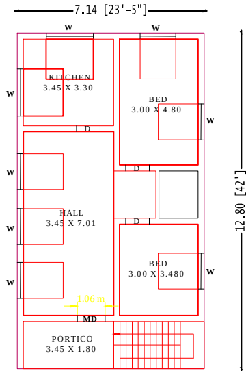
GROUND FLOOR PLAN (NOTH FACING)
