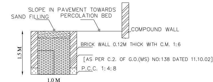
SECTION OF RAIN WATER PERCOLATION BED STAIR CASE DETAILS: -
