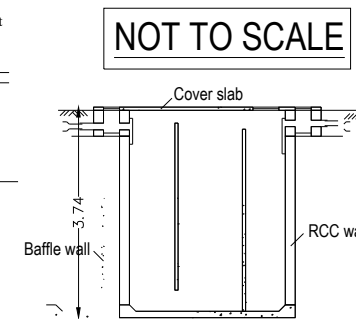
SECTION OF SEPTIC TANK
