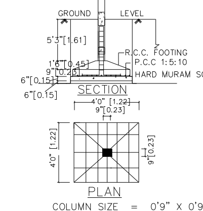
PLAIN COLUMN SIZE = 0'9" x 0'9"
