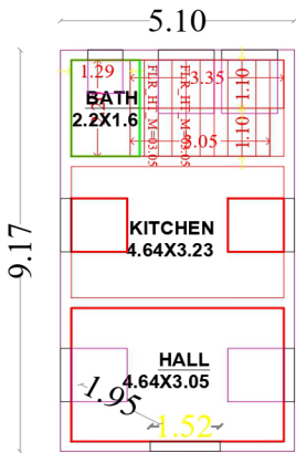
GROUND FLOOR PLAN (FACEING OF NORTH)
